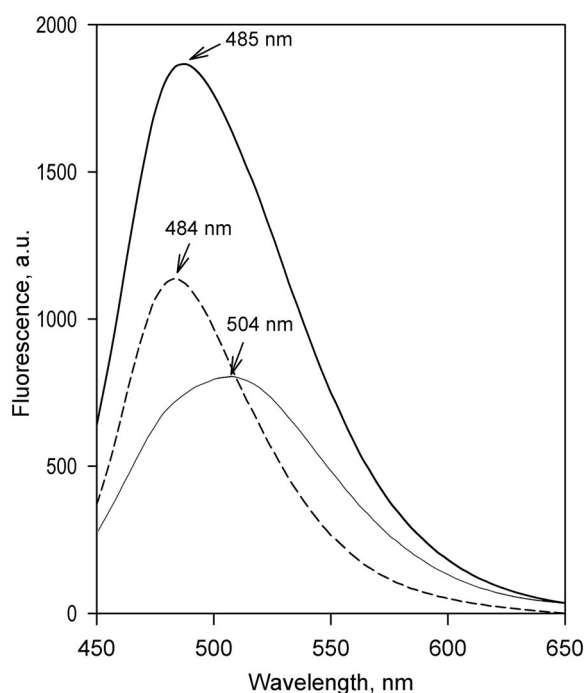
Figure 3. Fluorescence of Coumarin 152 and Coumarin 151. The graph shows the spectra of emission of 1 \mu\text{M} C152 (solid line) and C151 (thin solid line) in 0.1 \text{ M} Na-Hepes buffer, pH 7.4, containing 60 \text{ mM} KCl in the presence of HLM-2 ( 0.33 \text{ mg protein/mL} ). The dashed line shows the difference between the spectra of emission of C152 and C151.
