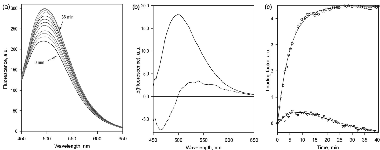
Figure 2. Changes in fluorescence resulting from the metabolism of C152 by HLM. Panel a shows a series of spectra of fluorescence recorded at 0, 0.75, 1.5, 1.25, 3.75, 4.5, 6, 12, 24, and 36 min after adding NADPH to the reaction mixture containing HLM (0.076 \mu\text{M} by the content of CPR) and 29 \mu\text{M} C152. Panels b and c show respectively the spectra and the loading factors of the first (solid line, circles) and the second (dashed line, triangles) principal components derived from the application of PCA to the series of spectra shown in panel a. The lines shown in panel c represent approximations of the time dependencies of the loading factors with a bi-exponential equation. These approximations are displayed solely to emphasize the general trend of the observed changes and have no interpretational value.
