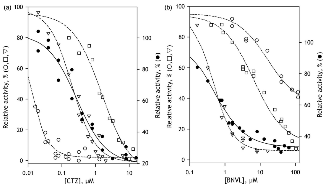
Figure 8. Inhibition of C152 demethylation by clotrimazole (a) and (+)-N-3-benzylirvanol (b). The results obtained with SS(3A4), SS(2C19), and SS(2B6) are shown in open circles, triangles, and squares, respectively. The results obtained with HLM are shown in closed circles. The datasets exemplified in the plots represent combinations of 2–4 individual experiments. The lines (dashed for Supersomes and solid for HLM) show the approximations of the datasets with Eq. 1. The ordinates for the datasets obtained with HLM are shifted down for better clarity of the graphs.
