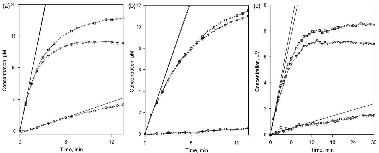
Figure 7. Kinetics of accumulation of the products of C152 metabolism derived from the application of PCA to the results of experiments with scanning fluorimetry. Panels a , b and c represent the results obtained with SS(2B6), SS(3A4), and HLM, respectively. The concentrations of Supersomes and HLM in the incubation mixture were equal to 0.076 \mu\text{M} P450 and 1.5 \text{ mg protein/mL} (or 0.076 \mu\text{M} CPR), respectively. The plots show the kinetic curves of the changes in the concentrations of DC152 (triangles), C151 (circles), and the total of the two products (squares) obtained from the results of PCA. Solid lines illustrate the initial velocities of product accumulation derived from the approximation of the initial fragments of the kinetic curves with the first or second-order polynomial.
