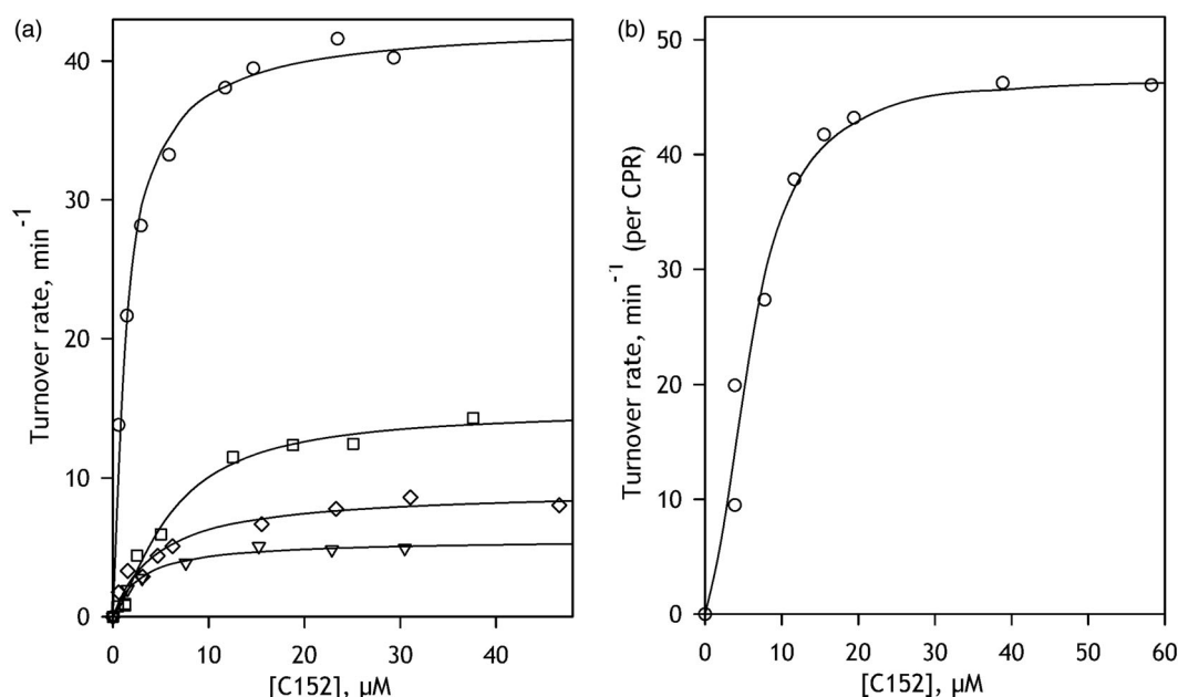
Figure 4. Dependencies of the rate of C152 metabolism on substrate concentration. Panel a shows the representative datasets obtained with SS(2B6) (circles), SS(3A4) (squares), SS(1A2) (triangles) and SS(2C19) (diamonds). The results obtained with HLM are exemplified in panel b . The solid lines represent the results of fitting of the datasets to the Hill (HLM and SS(3A4)) or Michaelis-Menten (SS(2B6), SS(1A2), and SS(2C19)) equations.
