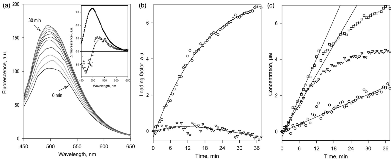
Figure 6. Analysis of the kinetics of accumulation of two sequential products of C152 metabolism with scanning fluorimetry and PCA. Panel a shows a series of spectra of fluorescence recorded in 3 min intervals during the incubation of SS(1A2) ( 0.076 \mu\text{M} P450) with 29 \mu\text{M} C152 in the presence of NADPH. The inset shows the spectra of the first (filled circles) and the second (open circles) principal components derived with PCA. Solid lines represent the approximations of these spectra with the prototypical spectra of fluorescence of DC152 and C151 (see Figure 5). Panel b shows the time dependencies of the respective loading factors. Solid lines shown in this panel represent the approximations of the time dependencies of the loading factors with a bi-exponential equation. These approximations are presented solely to emphasize the general trend of the observed changes and have no interpretational value. Panel c shows the kinetic curves of the changes in the concentrations of DC152 (triangles), C151 (circles), and the total of the two products (squares) obtained from the results of PCA. Solid lines illustrate the initial velocities of product accumulation derived from the approximation of the initial fragments of the kinetic curves with a first-order polynomial.
